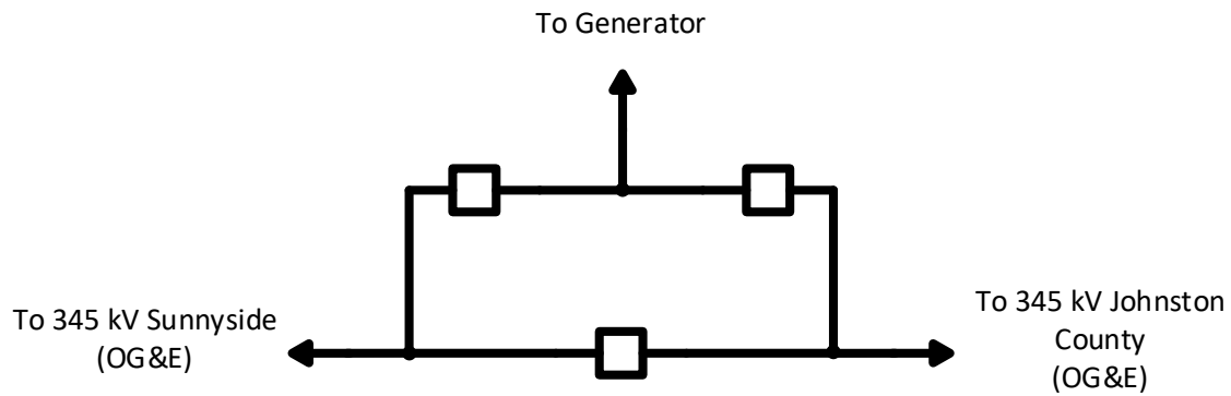
Figure 1: Point of Interconnection (POI INFORMATION) One-Line Diagram
